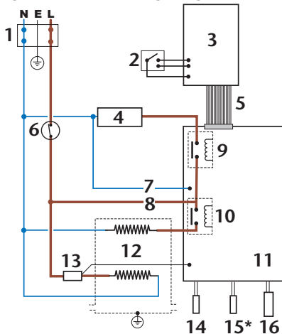
Fig.5 Shower Wiring Diagram
